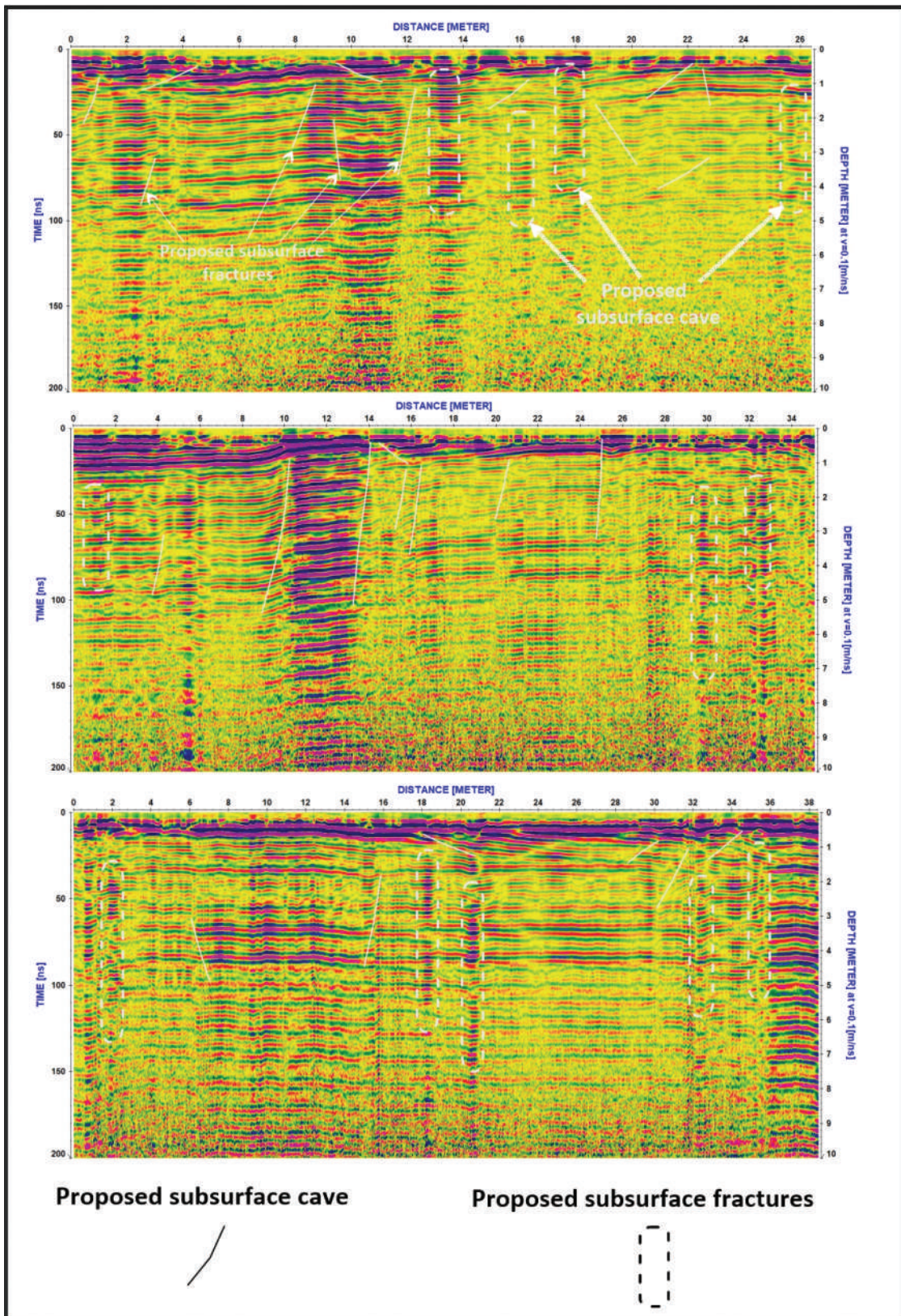
Figure 11. The 2D results of GPR scan with MALA system and 250 MHz antenna.
