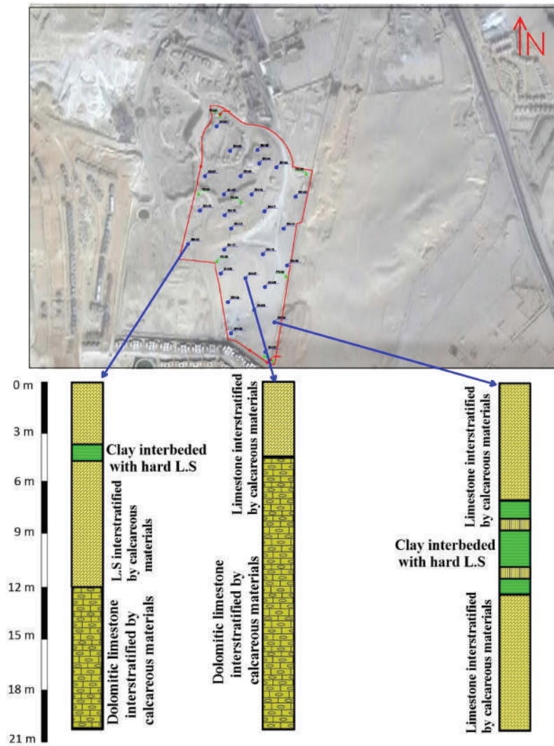
Figure 4. Drilled boreholes in the study area.
